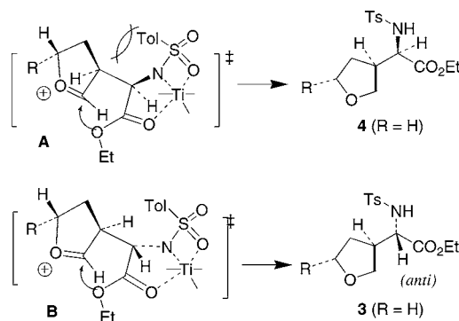
Figure 4. Stereochemical models.
