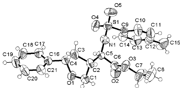
Figure 2. ORTEP drawing of X-ray structure of 13 .
