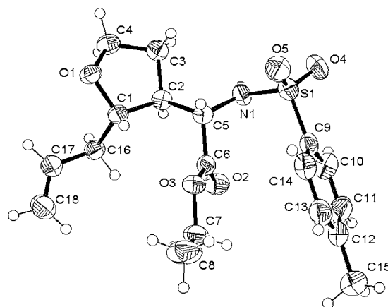
Figure 1. ORTEP drawing of X-ray structure of 5a .
